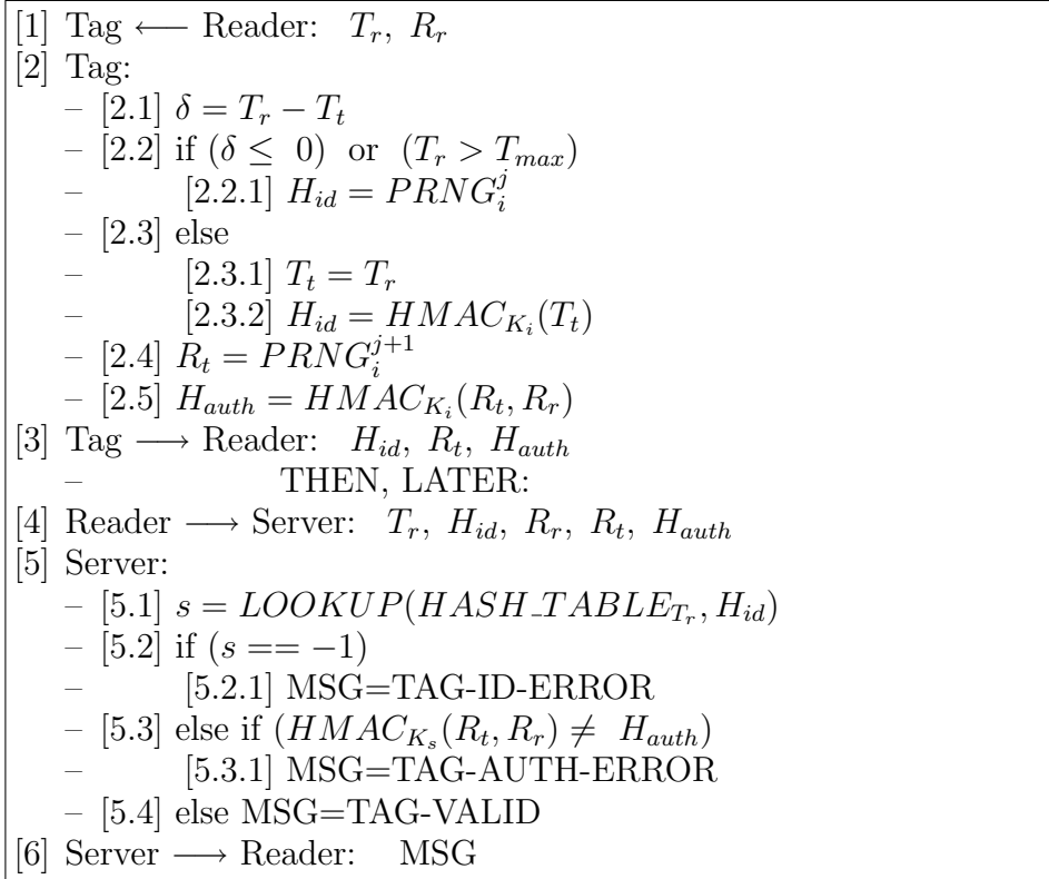
Fig. 2. YA-TRAP: Tag Authentication
